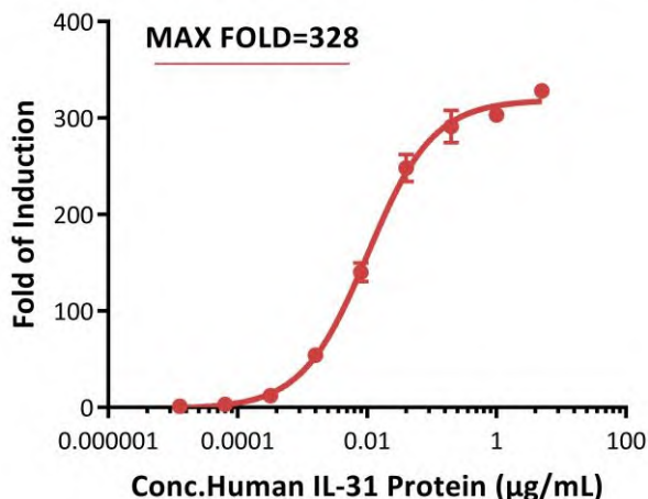
Fig3. Response to human IL-31 protein (FOLD). The Human IL-31 RA/OSMR (Luc) HEK293 Reporter Cell was stimulated with serial dilutions of human IL-31 protein (Cat. No. IL1-H5247). The max induction fold was approximately 328.
