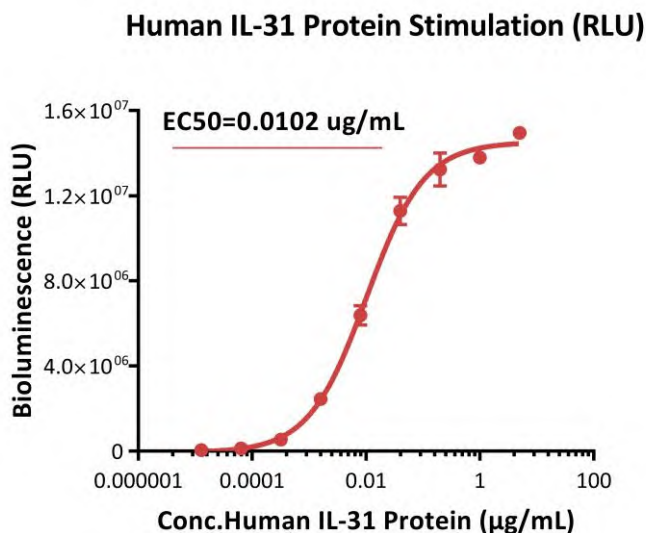
Fig2. Response to human IL-31 protein (RLU). The Human IL-31 RA/OSMR (Luc) HEK293 Reporter Cell was stimulated with serial dilutions of human IL-31 protein (Cat. No. IL1-H5247). The EC50 was approximately 0.0102 µg/mL.
